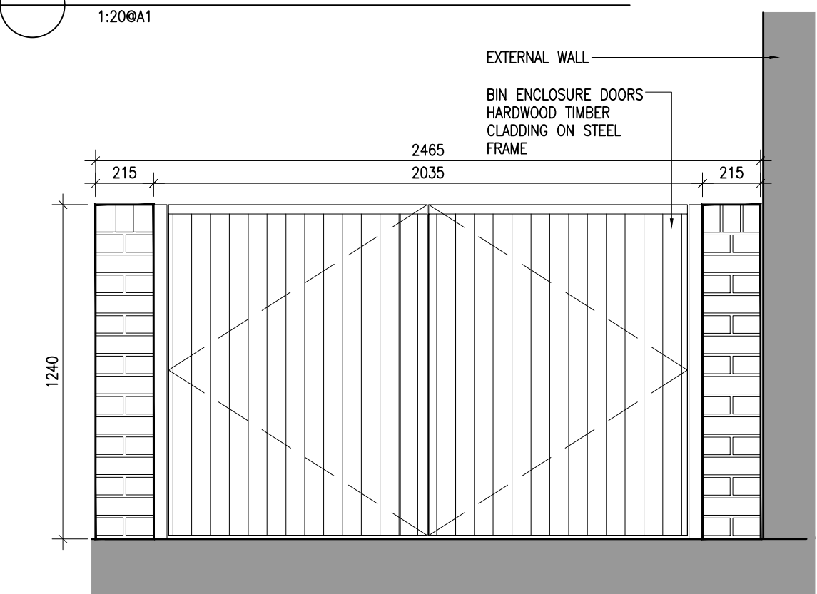
2 BIN STORE TYPE 1 FRONT ELEVATION 1:20@A1
