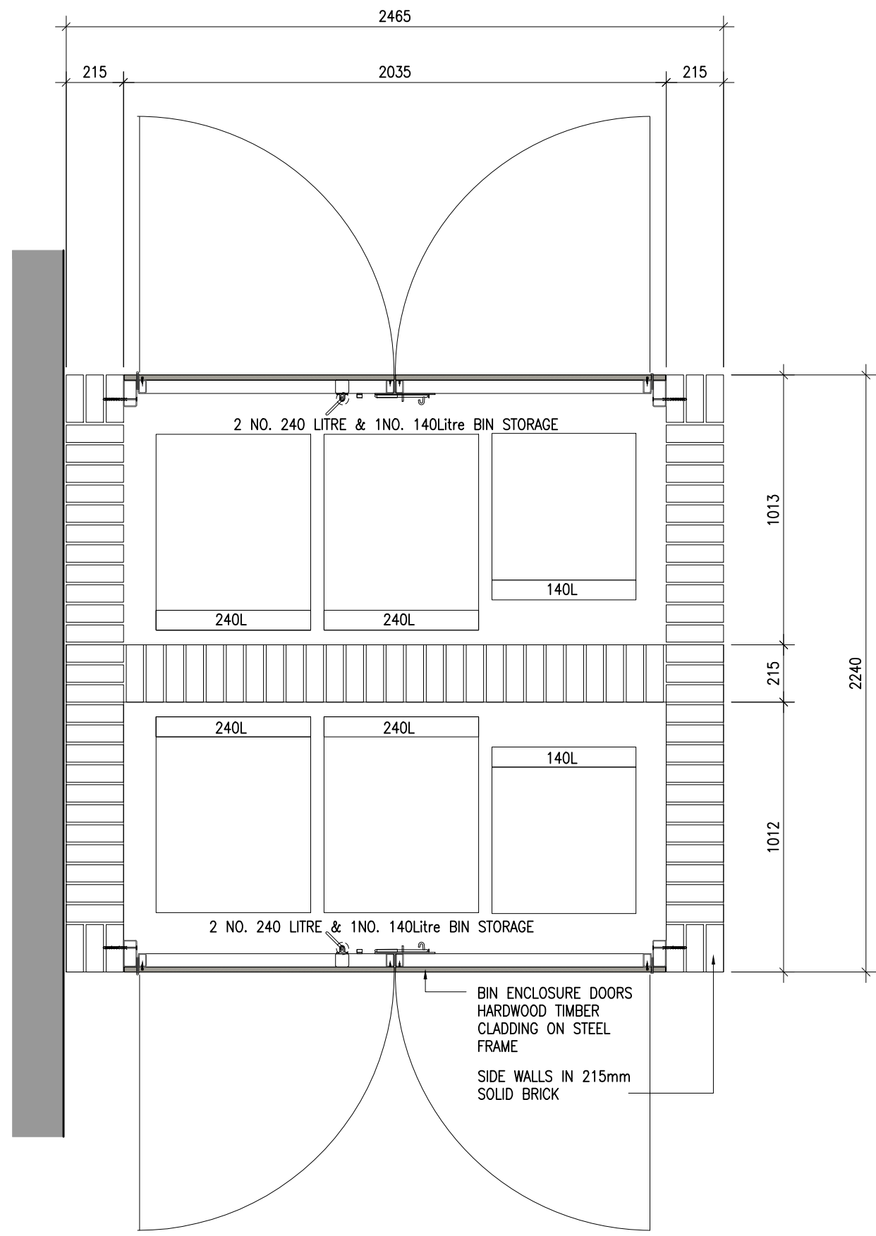
5 BIN STORE TYPE 2 PLAN 1:20@A1
