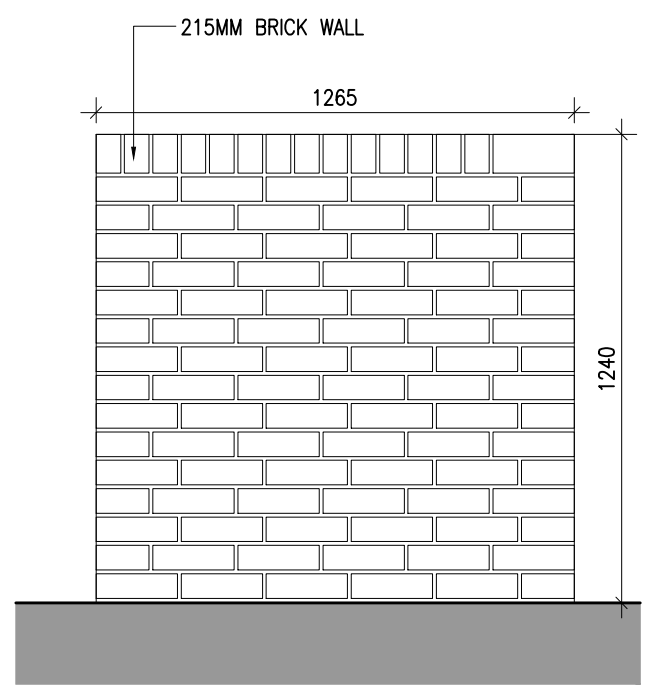
4 BIN STORE TYPE 1 SIDE ELEVATION 1:20@A1
