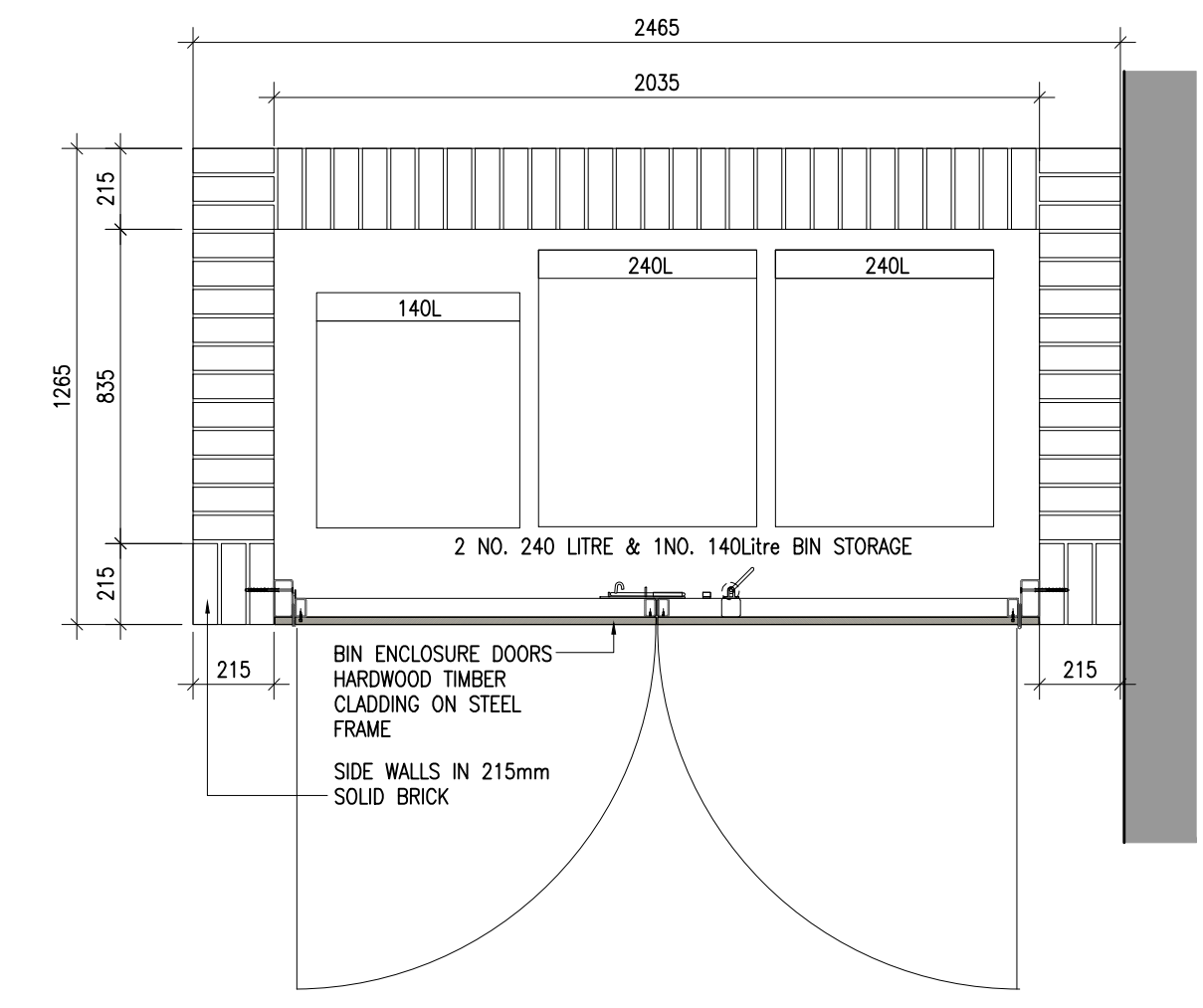
1 BIN STORE TYPE 1 PLAN 1:20@A1
