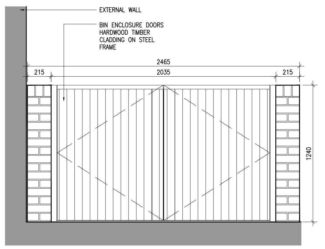
6 BIN STORE TYPE 2 FRONT ELEVATION 1:20@A1
