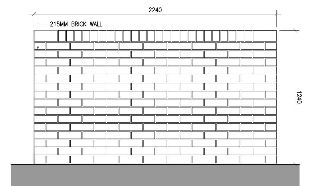
7 BIN STORE TYPE 2 SIDE ELEVATION 1:20@A1
